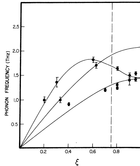
FIG. 2. Phonon frequencies for wave vector \vec{q} = (\xi, \xi, 0)/a , where a is the cubic lattice parameter; the dotted line is the zone boundary.
